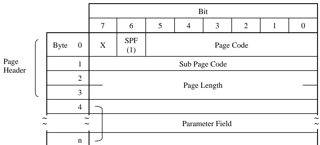
Figure 3.9 MODE SELECT command (Group 0) parameter configuration
