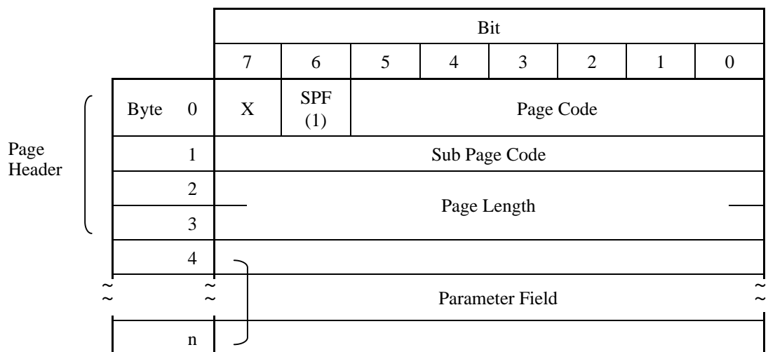
Figure 3.10 MODE SELECT EXTENDED command (Group 2) parameter configuration
