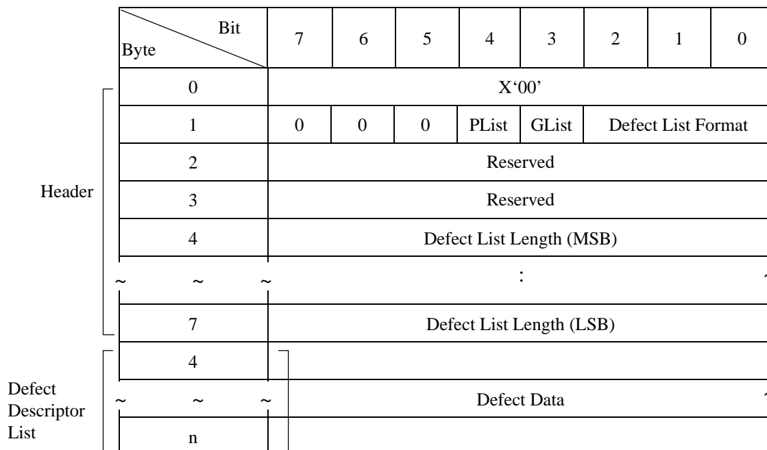
Figure 3.28 READ DEFECT DATA command (B7): Defect data configuration
