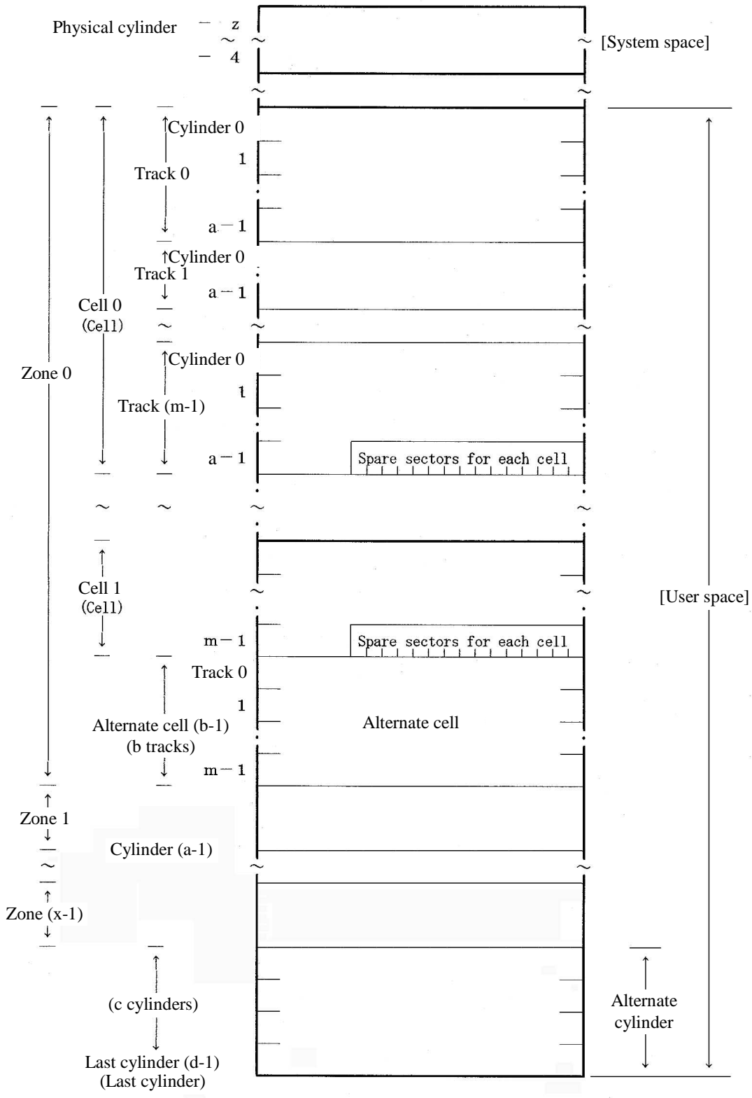
Figure 1.5 Data space configuration
