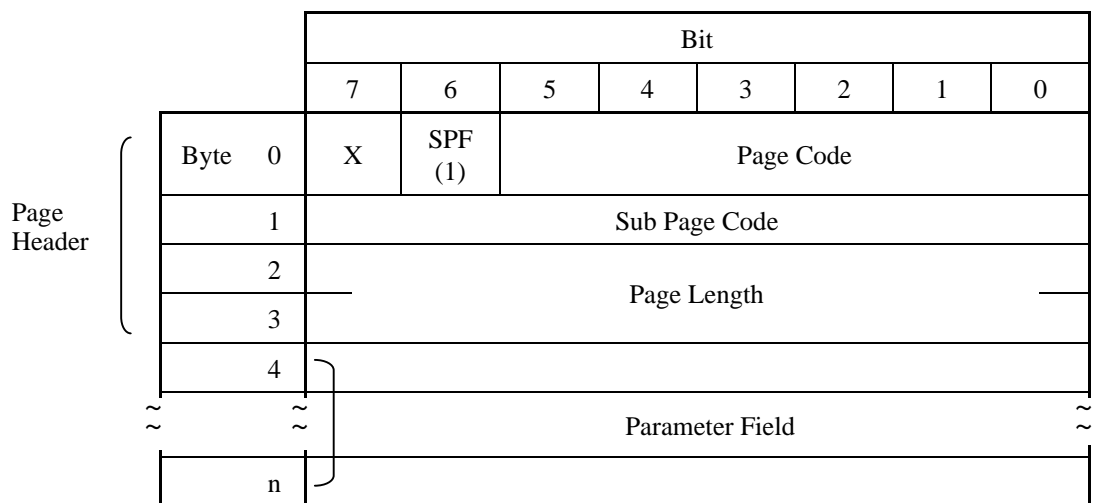
Figure 3.11 MODE SENSE command (Group 0) parameter configuration (2 of 2)
