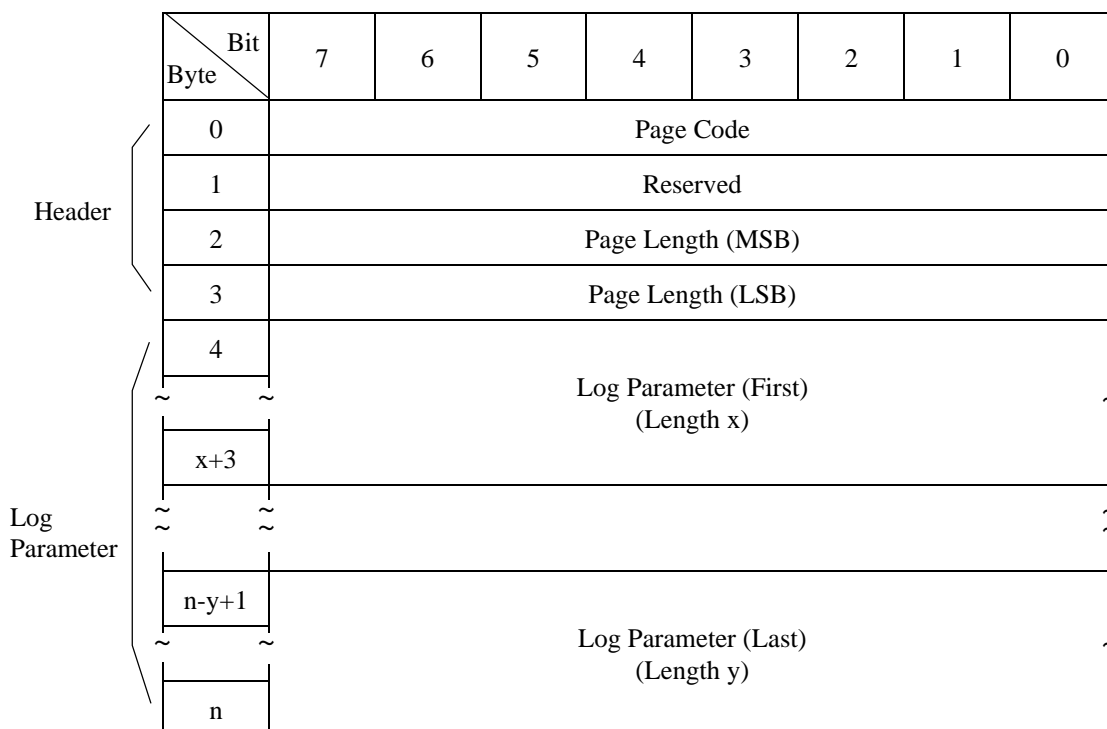
Figure 3.13 LOG, SELECT command: parameter list
