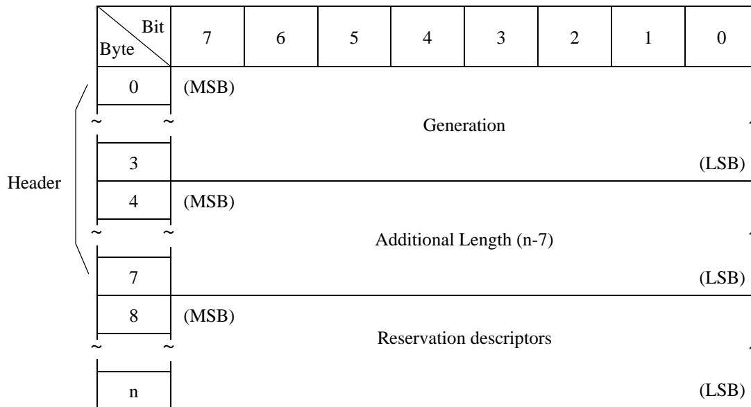
Figure 3.16 PERSISTENT RESERVE IN command: parameter data (READ RESERVATIONS)
