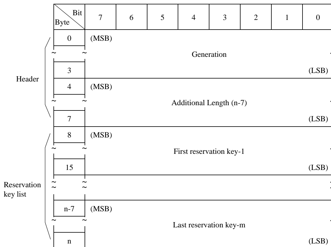
Figure 3.15 PERSISTENT RESERVE IN command: parameter data (READ KEYS)
