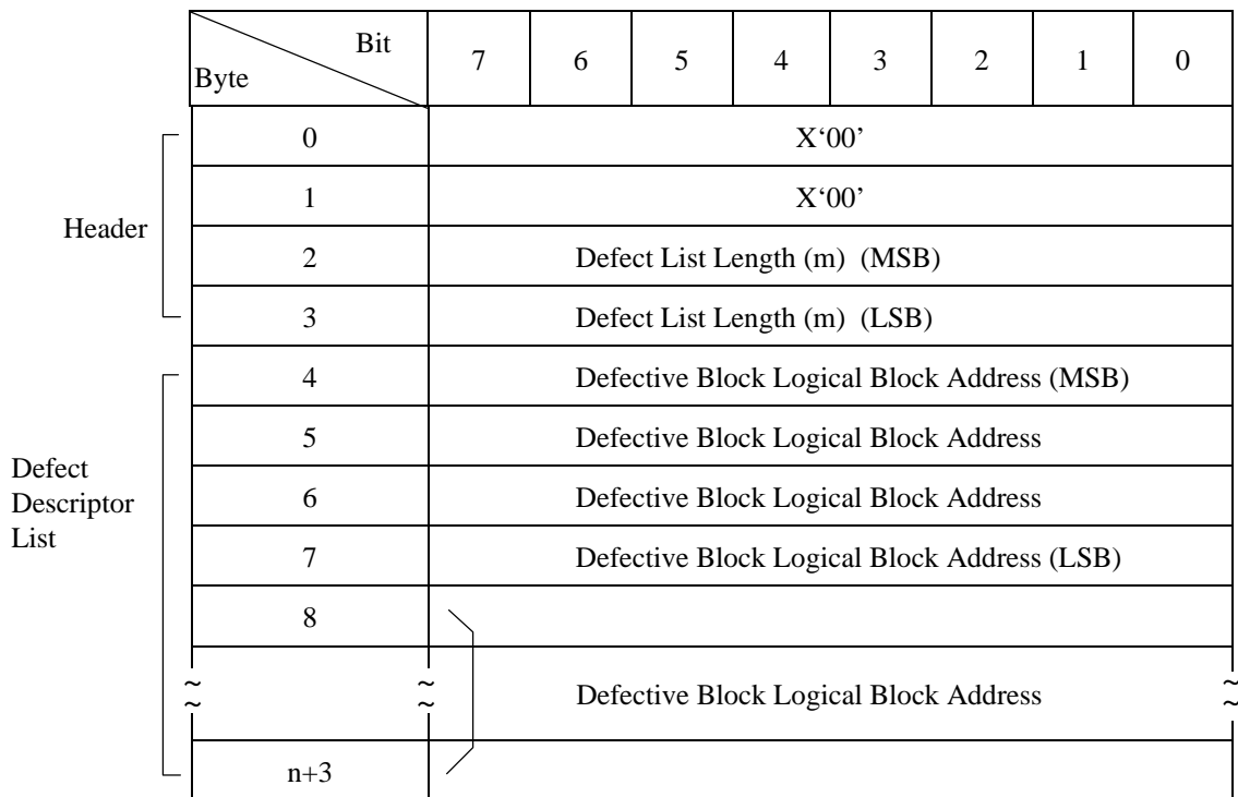
Figure 3.26 REASSIGN BLOCK command: defect data list configuration
