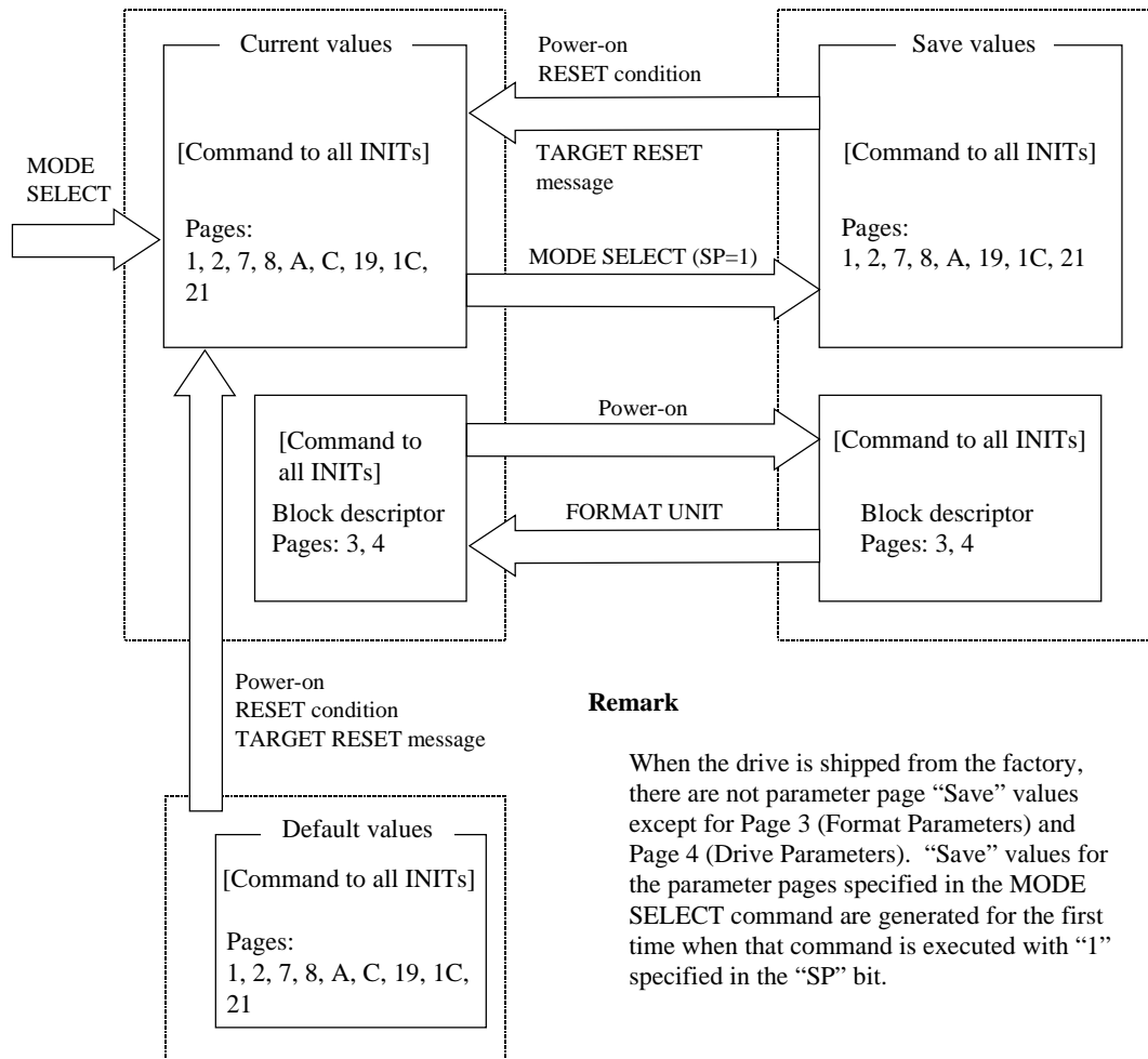
Figure 3.8 MODE SELECT parameter structure
