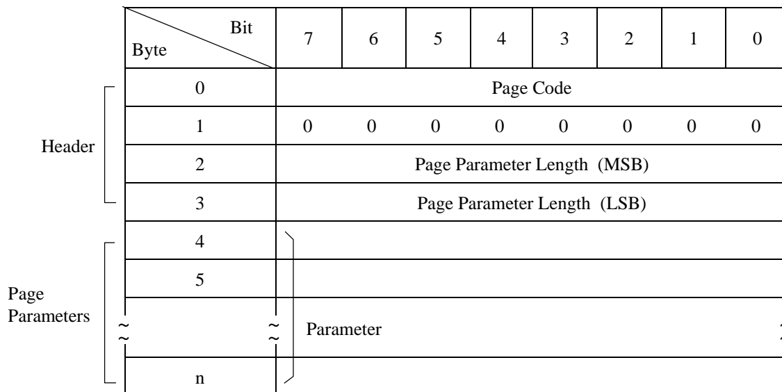
Figure 3.32 RECEIVE DIAGNOSTIC RESULTS command: Response data configuration
