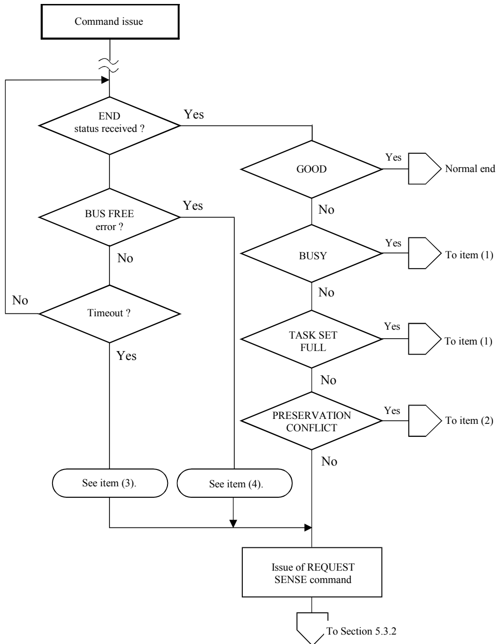
Figure 5.3 Analysis of the termination status
