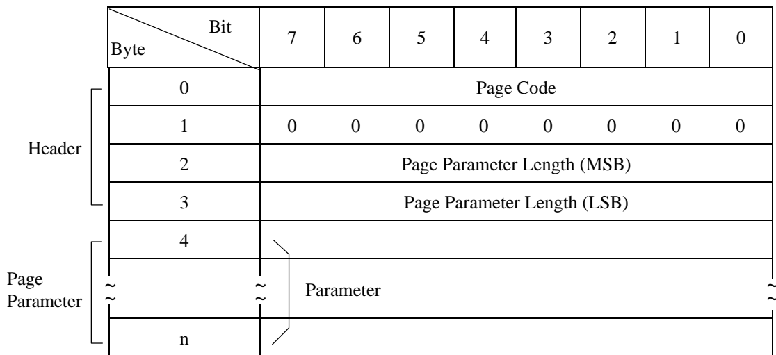
Figure 3.29 SEND DIAGNOSTIC command: parameter list configuration
