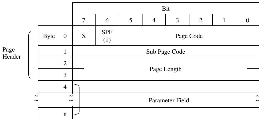
Figure 3.12 MODE SENSE EXTENDED command (Group 2) parameter configuration (2 of 2)
