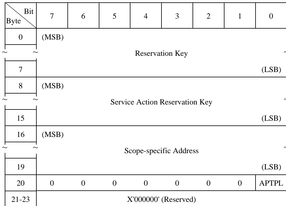
Figure 3.18 PERSISTENT RESERVE OUT command: parameter list
