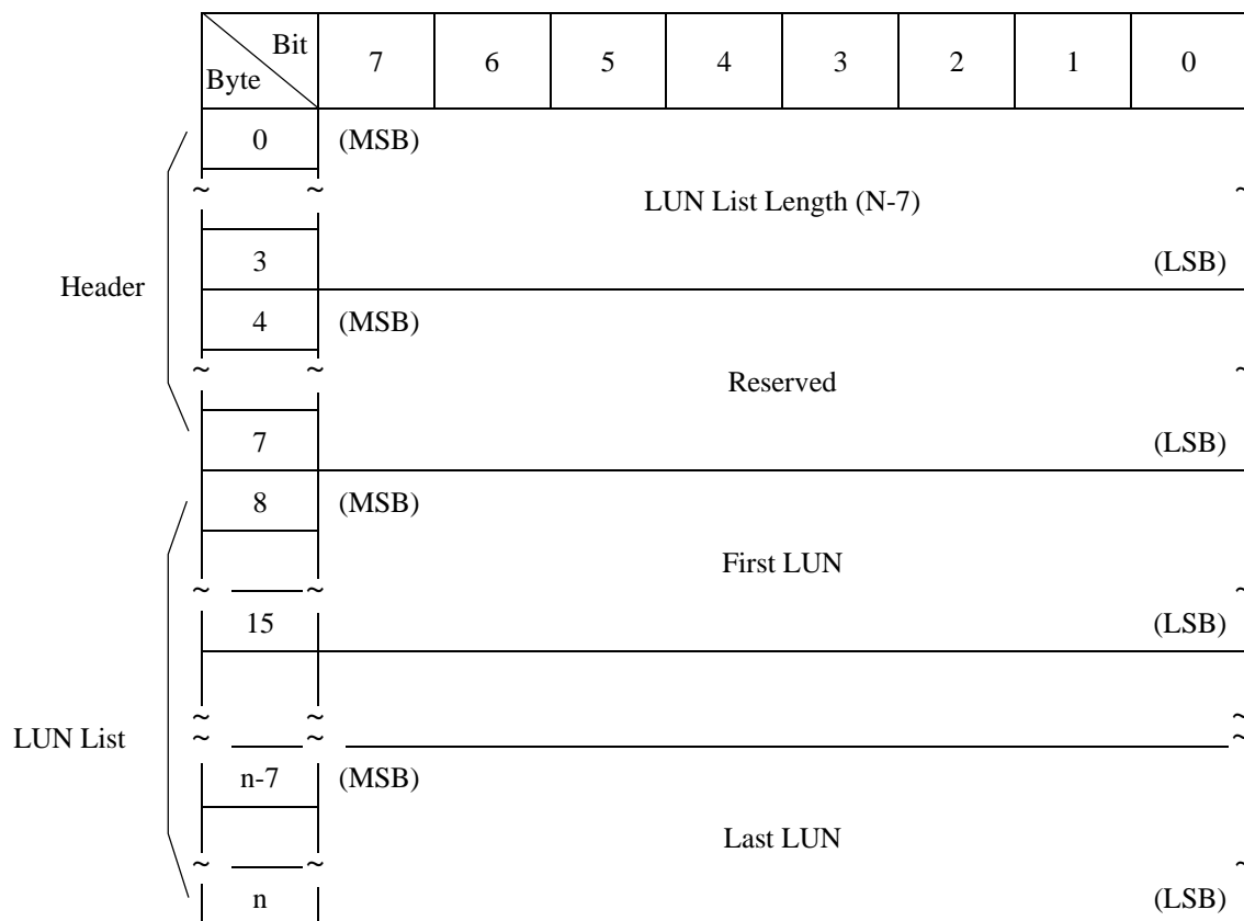
Figure 3.19 REPORT LUNS command: parameter list
