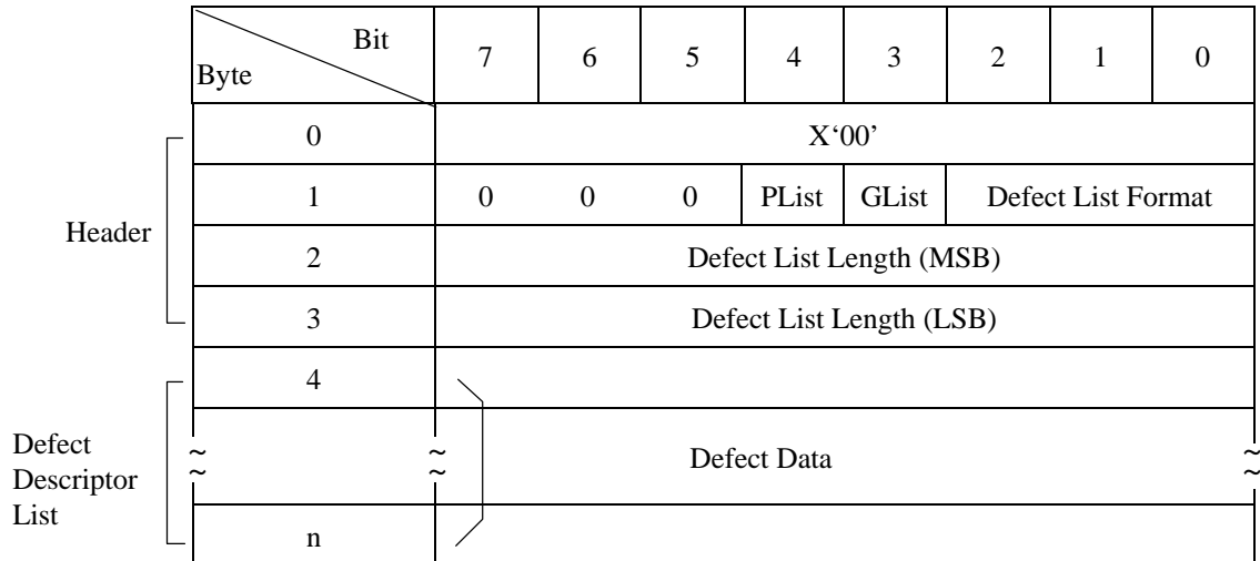
Figure 3.27 READ DEFECT DATA command (37): Defect data configuration
